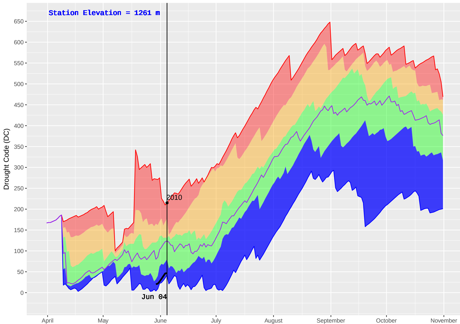
IDA BELL LAKE 3 (876) : Historical (2004–2016) and Current (2018) Noon Drought Code (DC)
