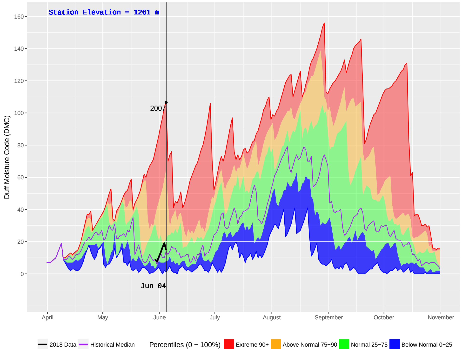
IDA BELL LAKE 3 (876) : Historical (2004–2016) and Current (2018) Noon Duff Moisture Code (DMC)
