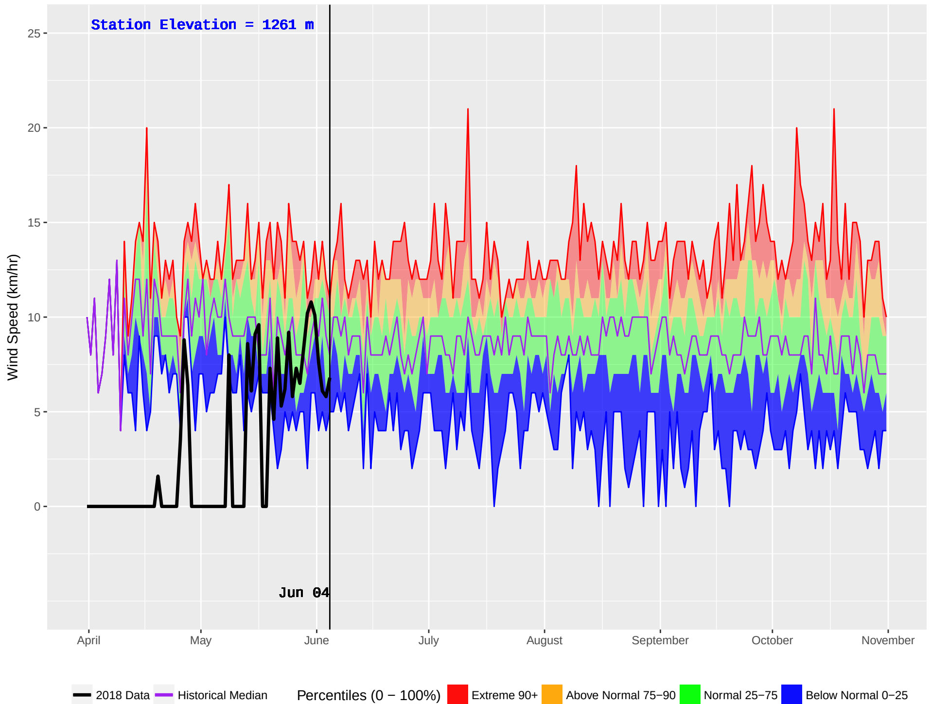
IDA BELL LAKE 3 (876) : Historical (2004–2016) and Current (2018) Noon Wind Speed
