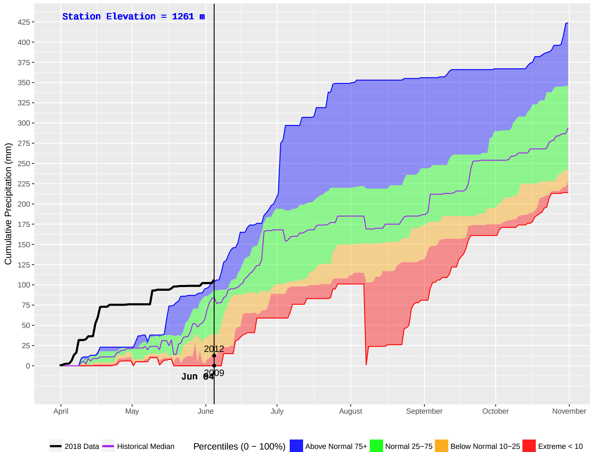
IDA BELL LAKE 3 (876) : Historical (2004–2016) and Current (2018) Noon Cumulative Precipitation
