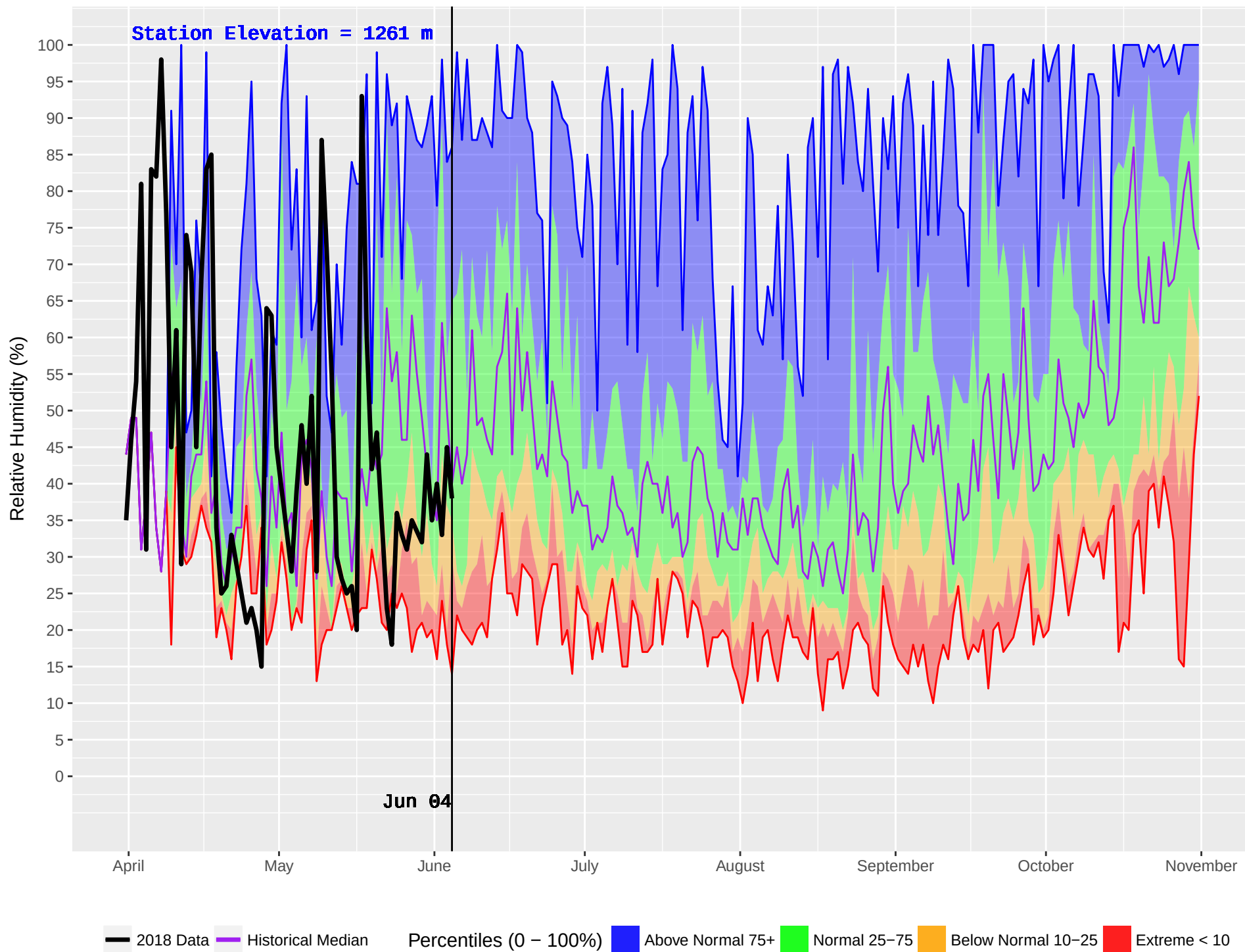
IDA BELL LAKE 3 (876) : Historical (2004–2016) and Current (2018) Noon Relative Humidity
