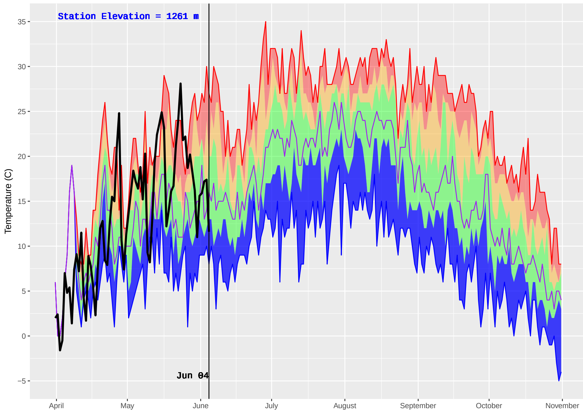
IDA BELL LAKE 3 (876) : Historical (2004–2016) and Current (2018) Noon Temperature
