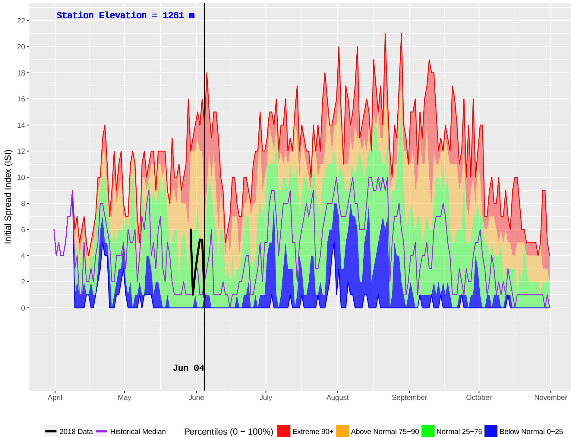
IDA BELL LAKE 3 (876) : Historical (2004–2016) and Current (2018) Noon Initial Spread Index (ISI)
