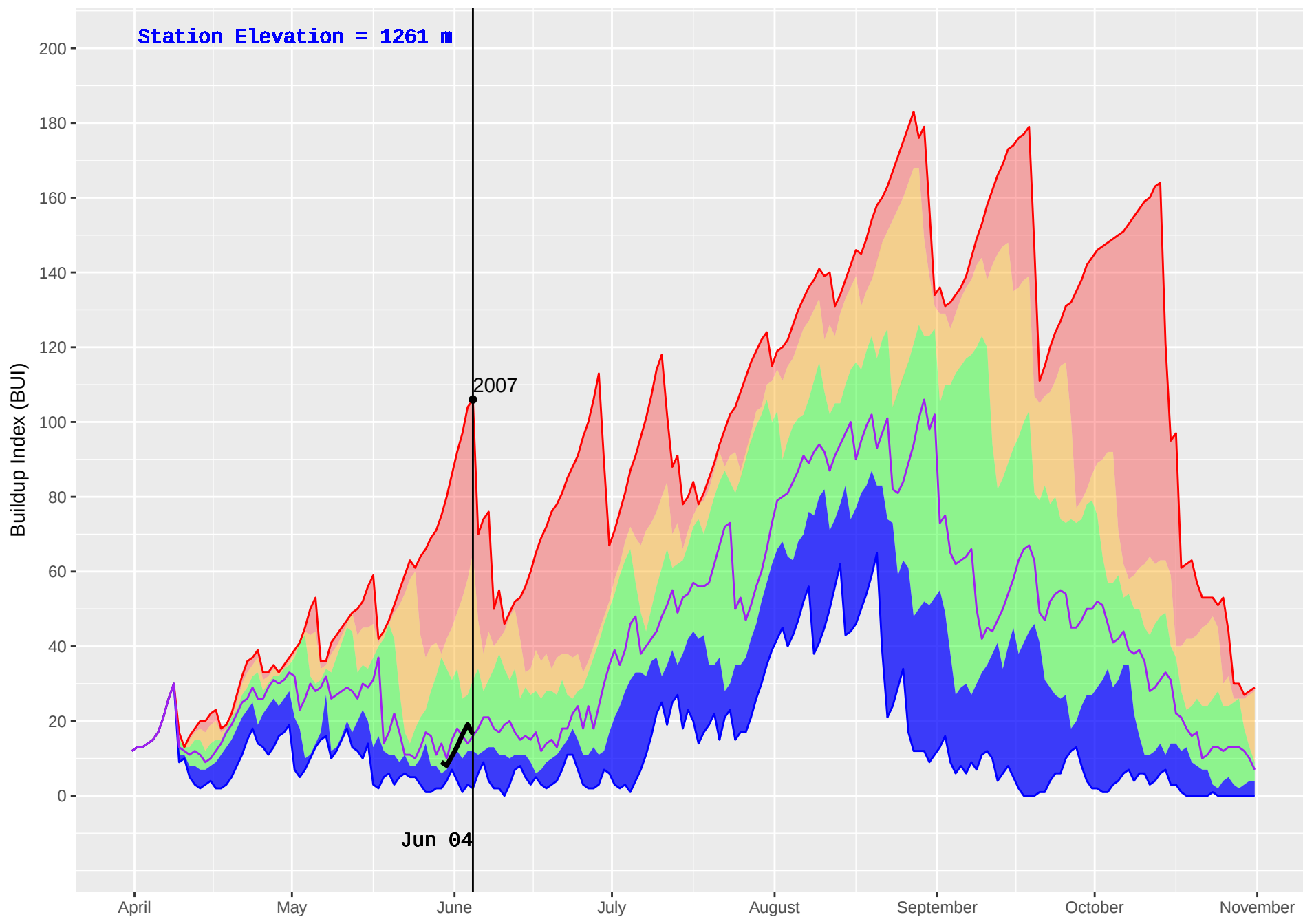
IDA BELL LAKE 3 (876) : Historical (2004–2016) and Current (2018) Noon Buildup Index (BUI)
